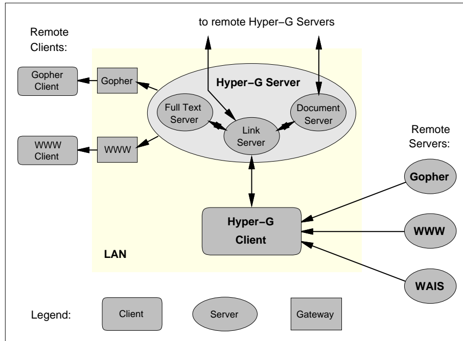
Fig. 1.: The architecture of Hyper-G
