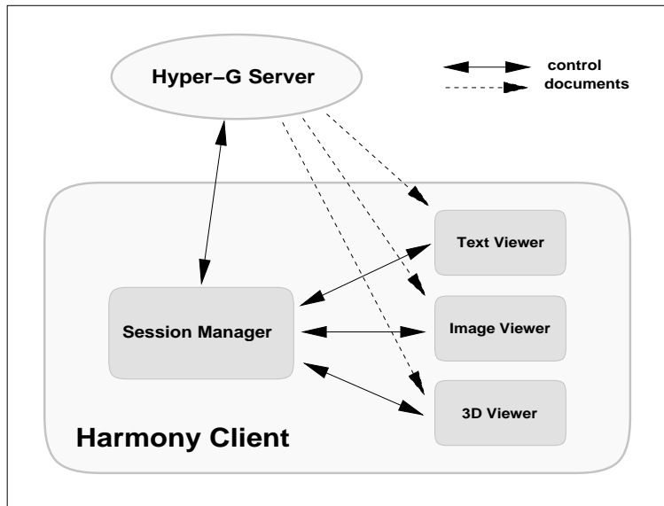
Fig. 2.: The architecture of Harmony
