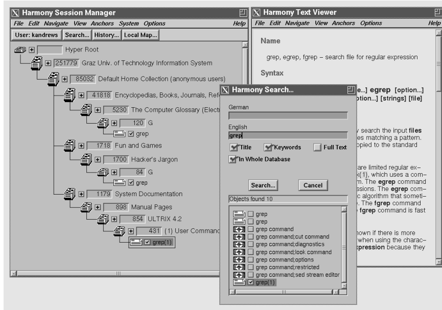
Fig. 5.: Harmony search dialogue
