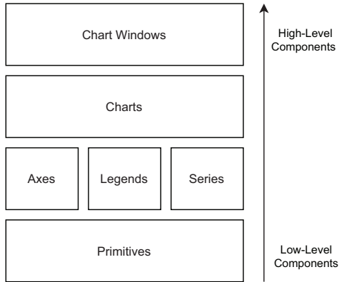
Fig. 2: The four layers of components in the RespVis library. Higher layers contain increasingly higher-level components.
